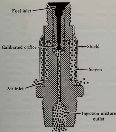
FIGURE 3-39. Fuel discharge nozzle.
